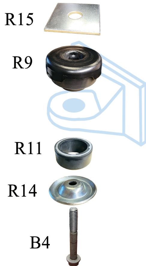
Cab Mounts
